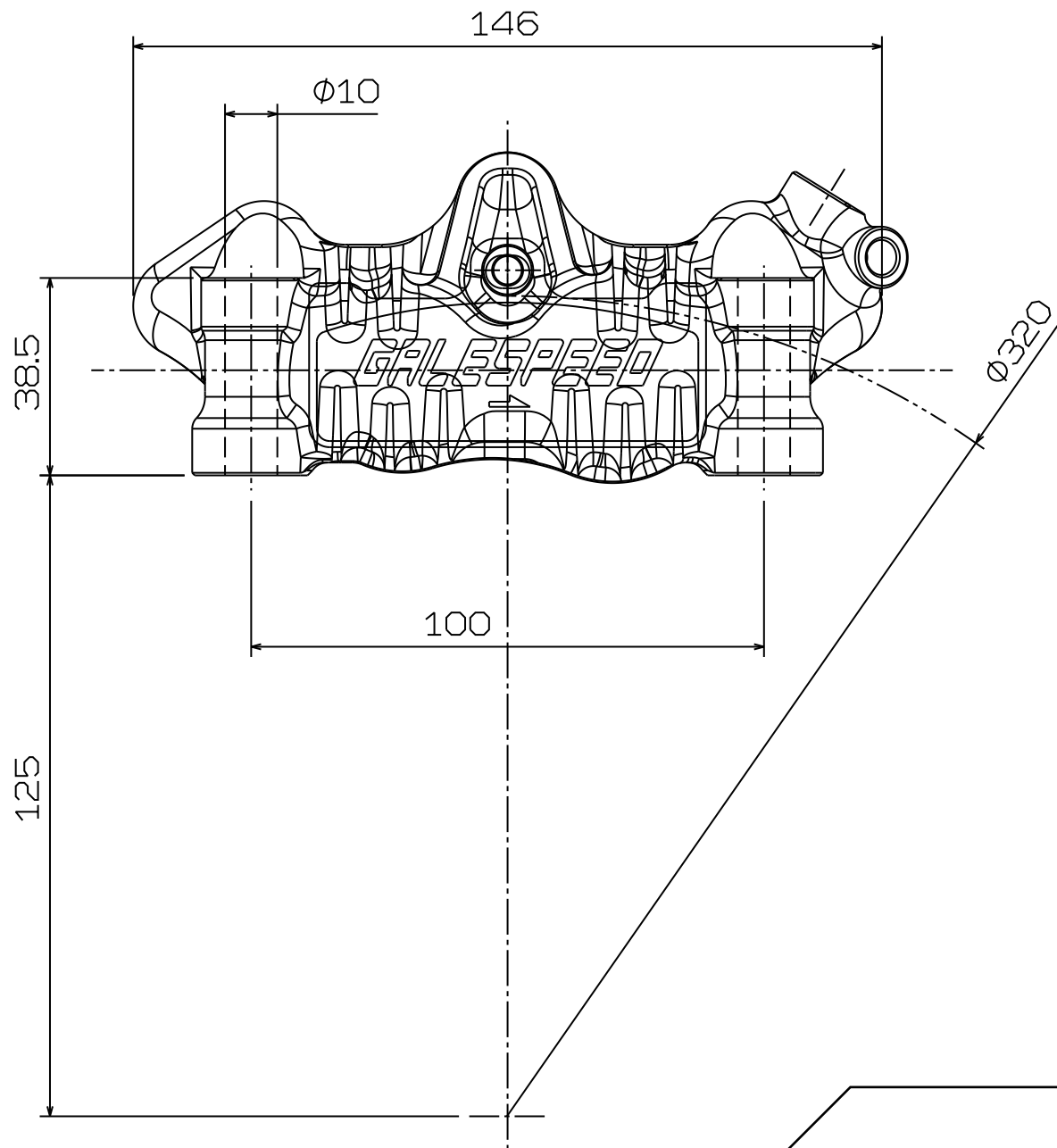
Front radial caliper 4 piston 100mm
